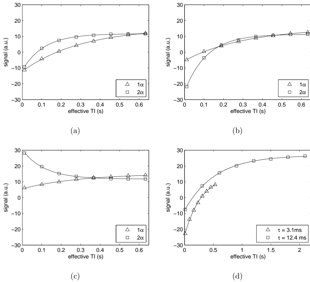
Figure 2.2: The transients measured in a sample with T_1 = 740 ms for the (a) DALL, (b) interleaved DALL, (c) non-inverted DALL and (d) D \tau LL flip angle mapping techniques. The nominal 1\alpha flip angle was 6^\circ . Solid lines are the curves fit to the data points in the flip angle analysis.
